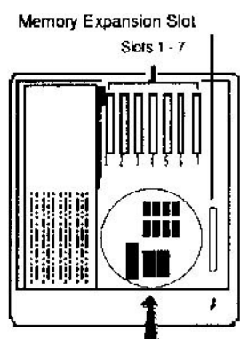
Rev 3 IIGS Motherboards 8 memory chips, 2 ROMs next to CPU
